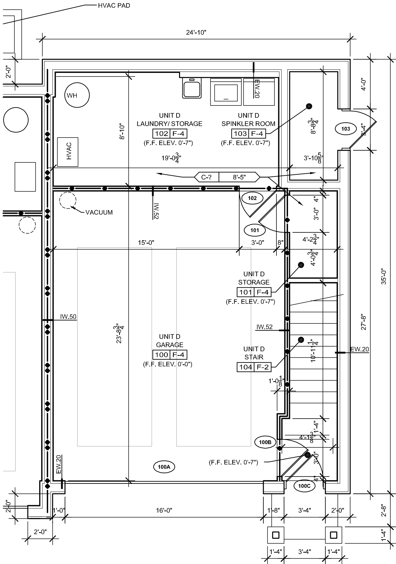
F5 LOWER LEVEL FLOOR PLAN (UNIT D) 1/4" = 1'-0"
