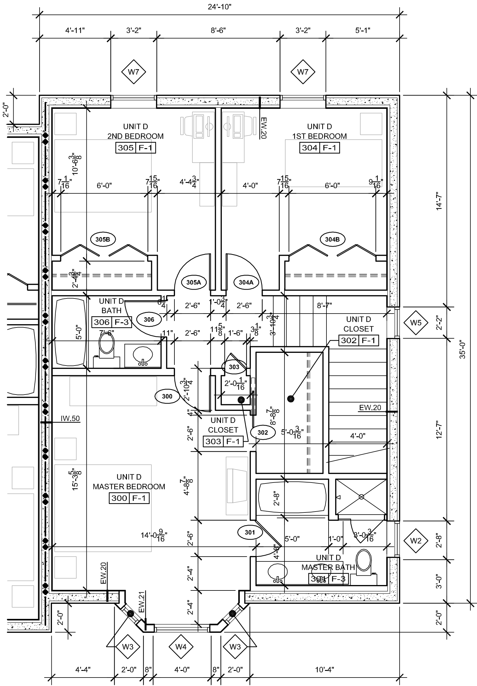
F1 UPPER LEVEL FLOOR PLAN (UNIT D) 1/4" = 1'-0" UNIT B SIM.; UNIT A & C SIM., OPP. HAND
