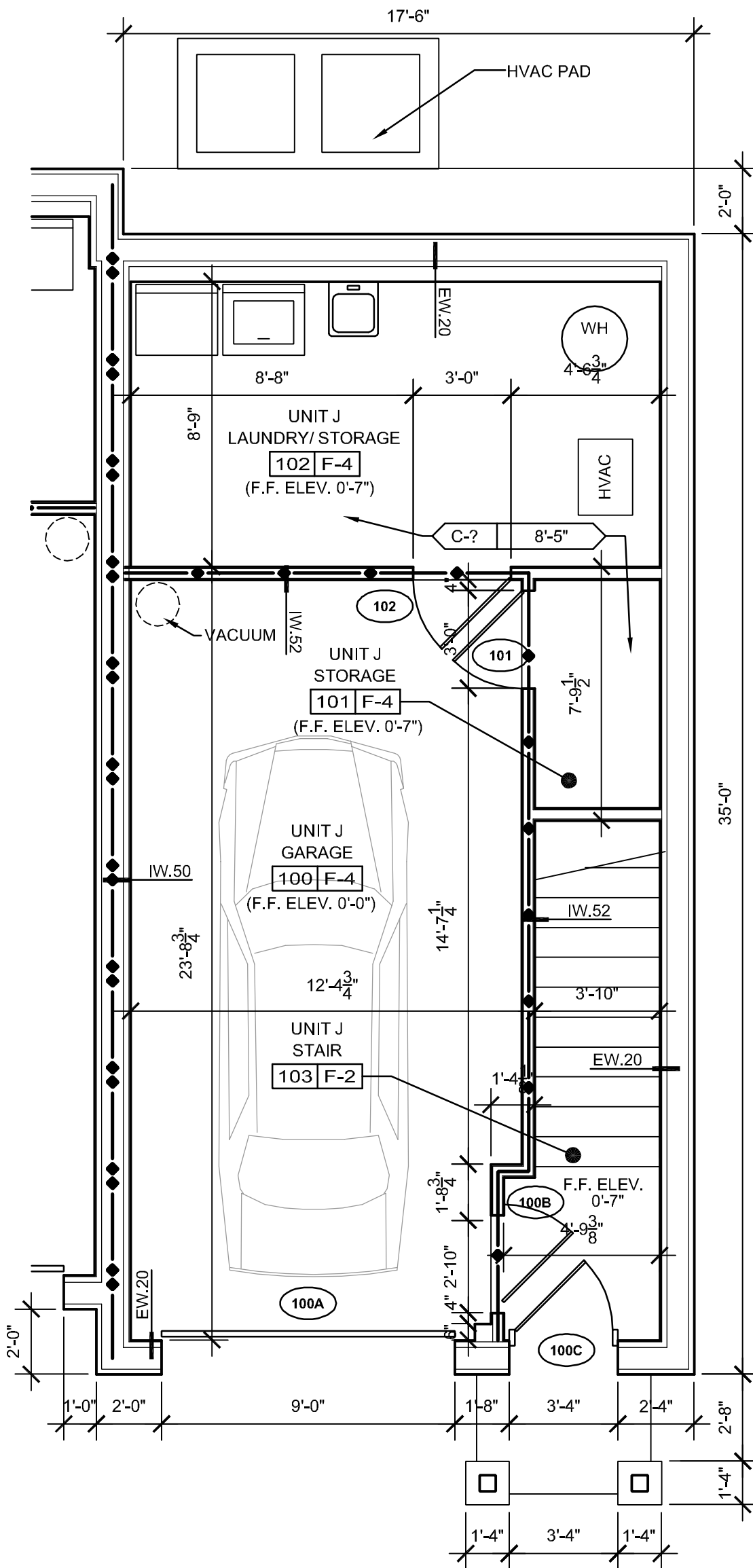
C4 LOWER LEVEL FLOOR PLAN (UNIT J) 1/4" = 1'-0" UNIT F & H SIM., UNITS E, G, & I SIM.; OPP. HAND
